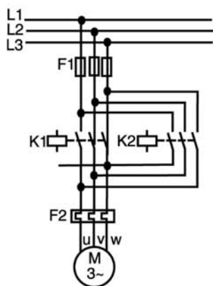
Circuito principal
